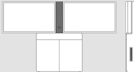
Media column EY-W8M2 – with 2 x 65" displays (also available as freestanding with floor plate)
